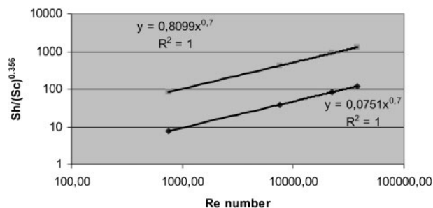
7 Variation of dimensionless corrosion rate, expressed as Sh number as function of Re number for two temperatures studied, a 20 (◇) and b 60°C (□)
